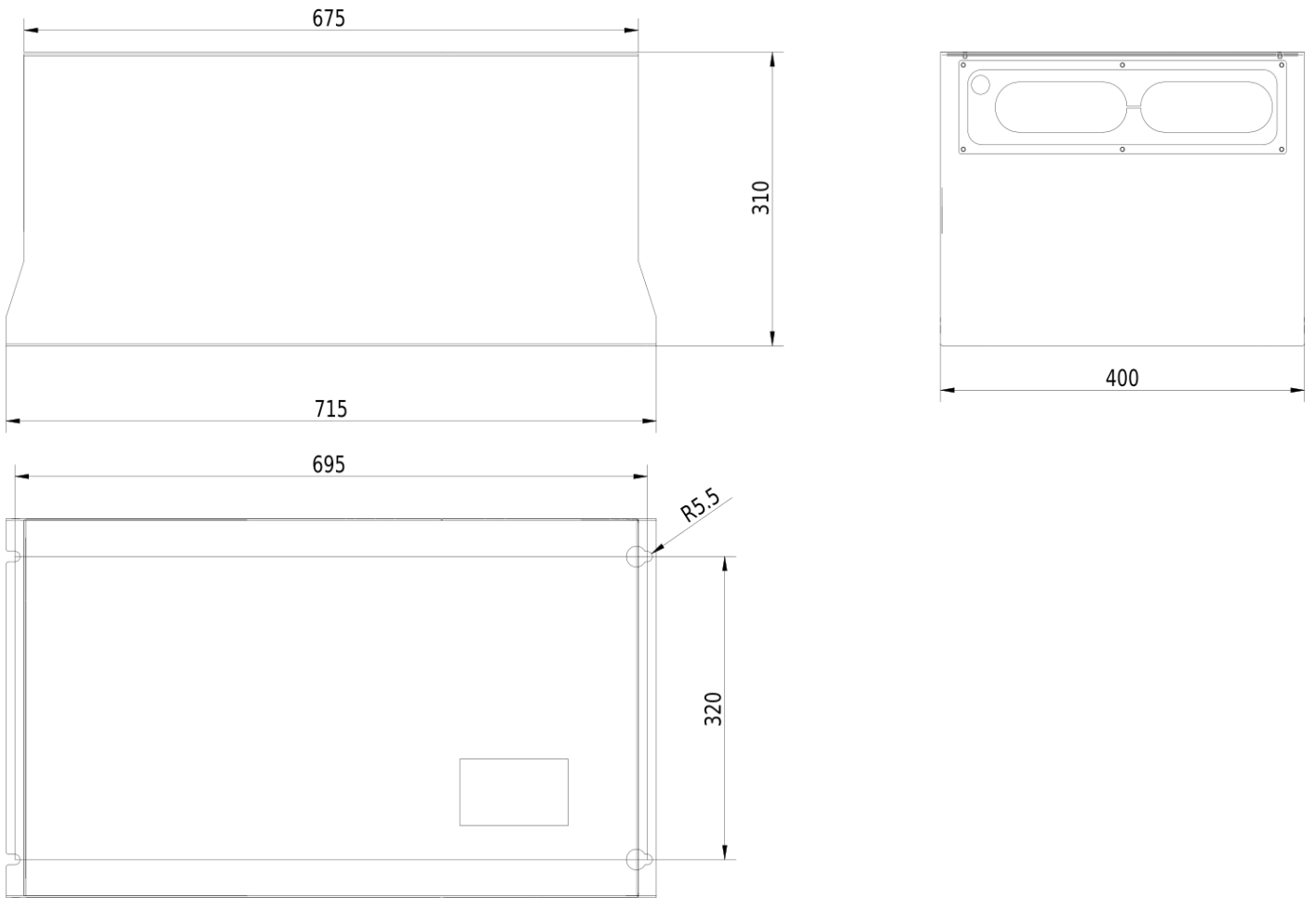
Dimensional drawing V900 - 160kW 4T1600
