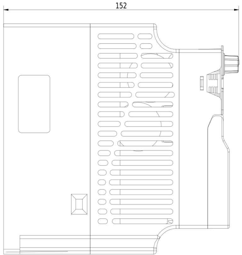
Dimensional drawing V800 - 2,2kW 4T0022
