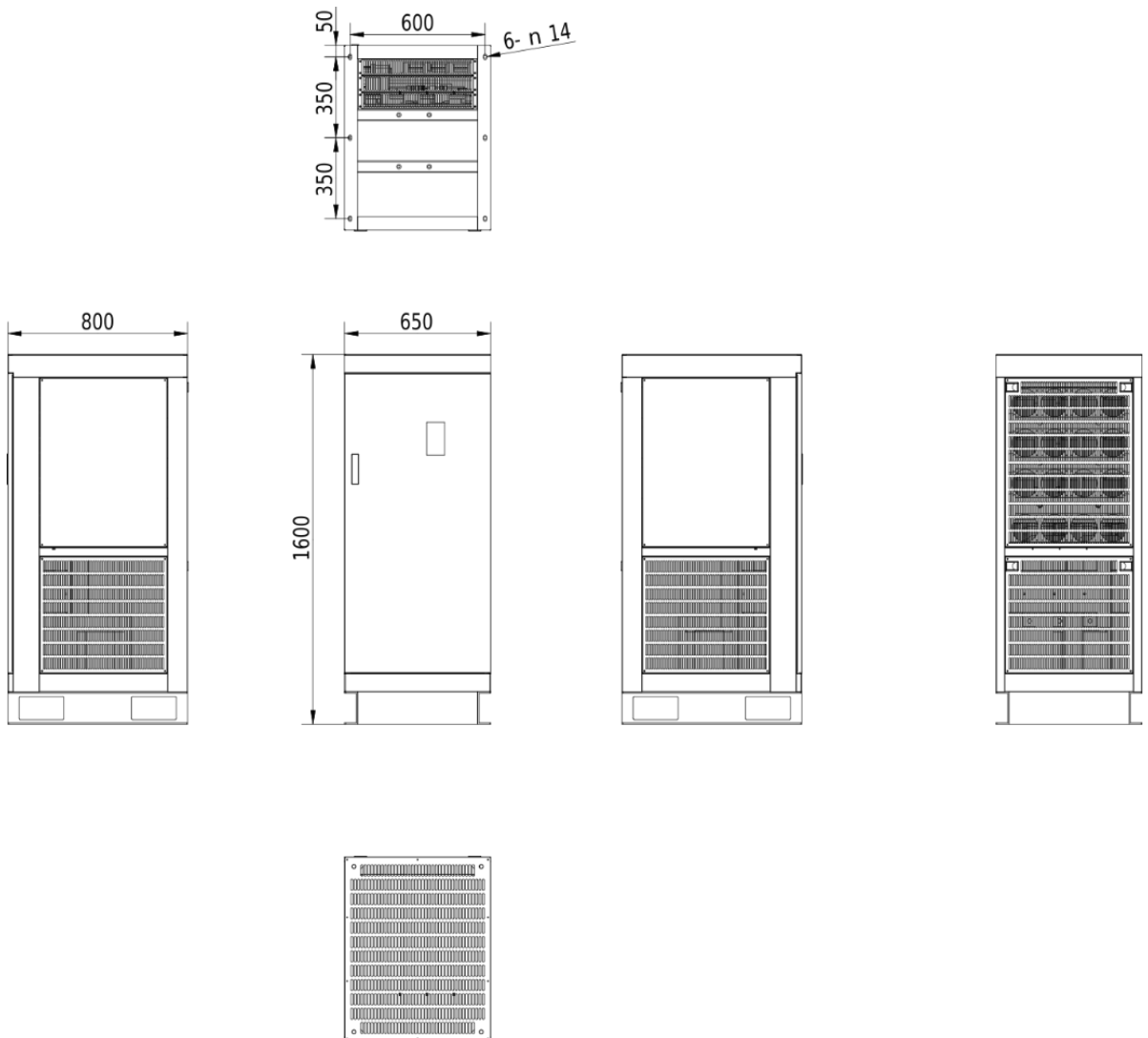
Dimensional drawing V810 - 630kW 4T6300
