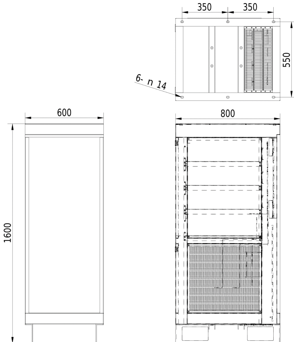
Dimensional drawing V810 - 400kW 4T4000
