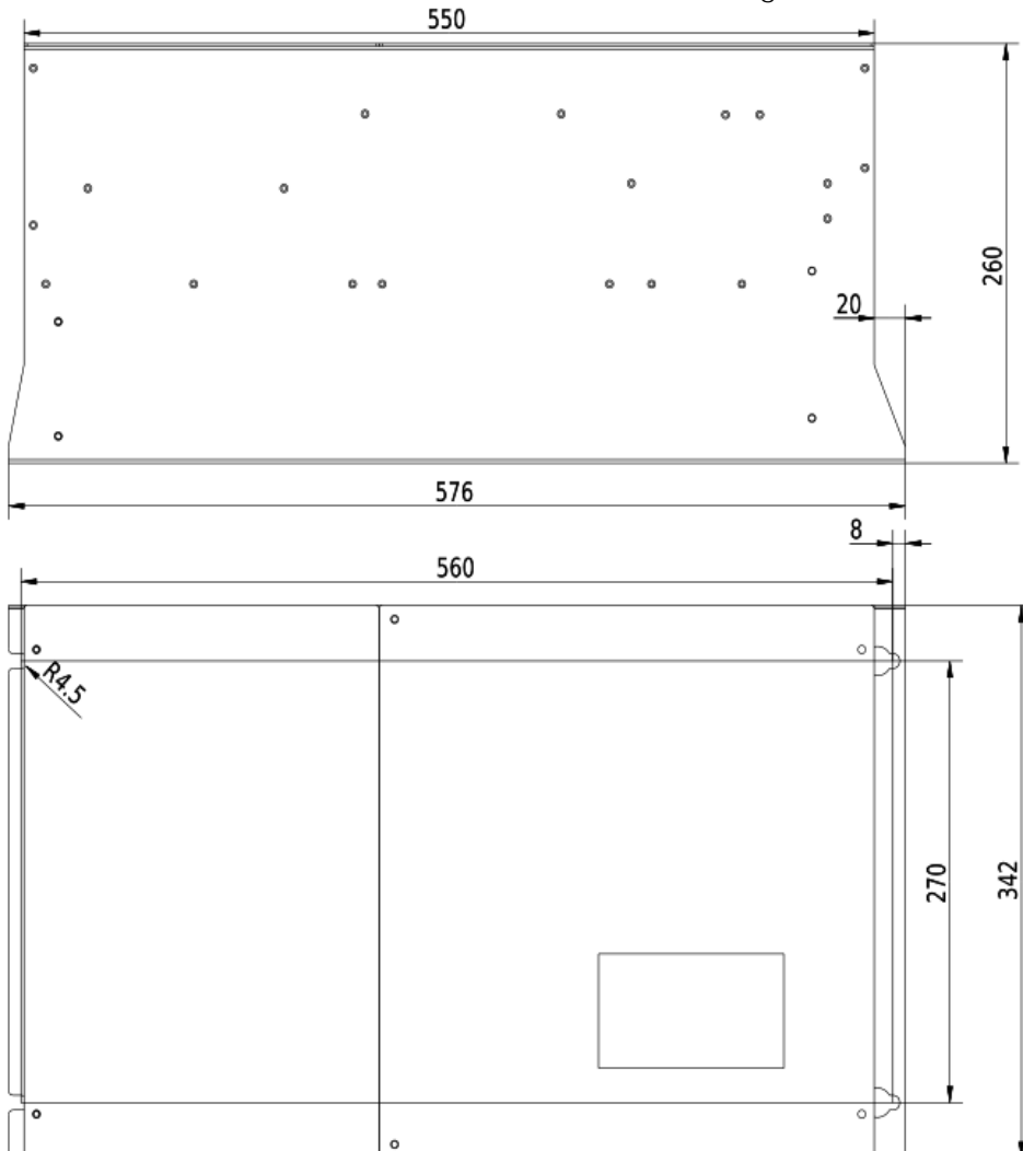
Dimensional drawing V810 - 132kW 4T1320
